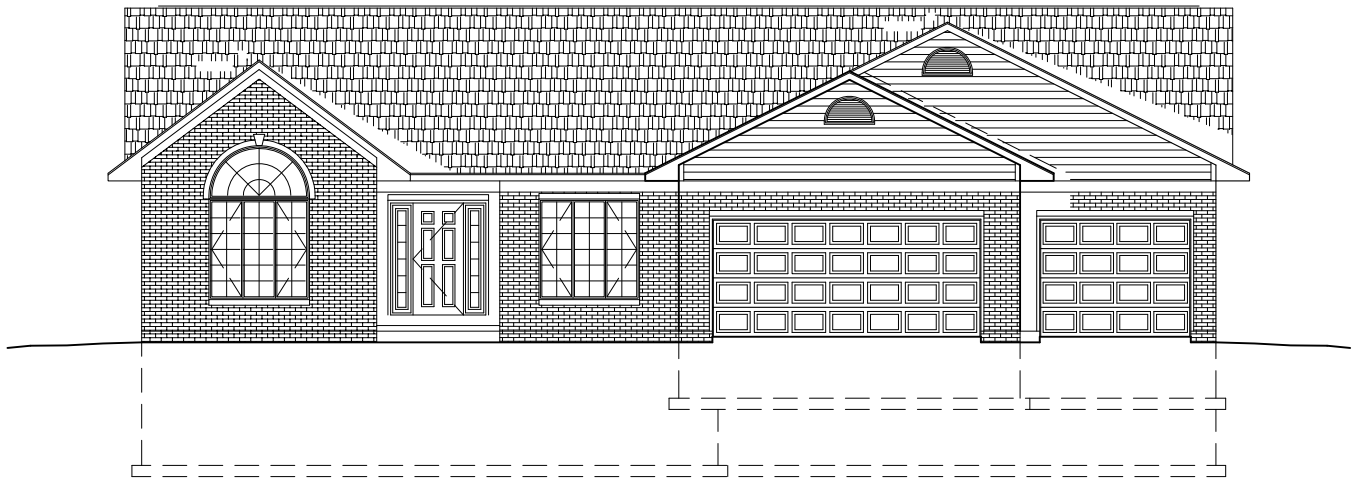
1 FRONT ELEVATION A-1
